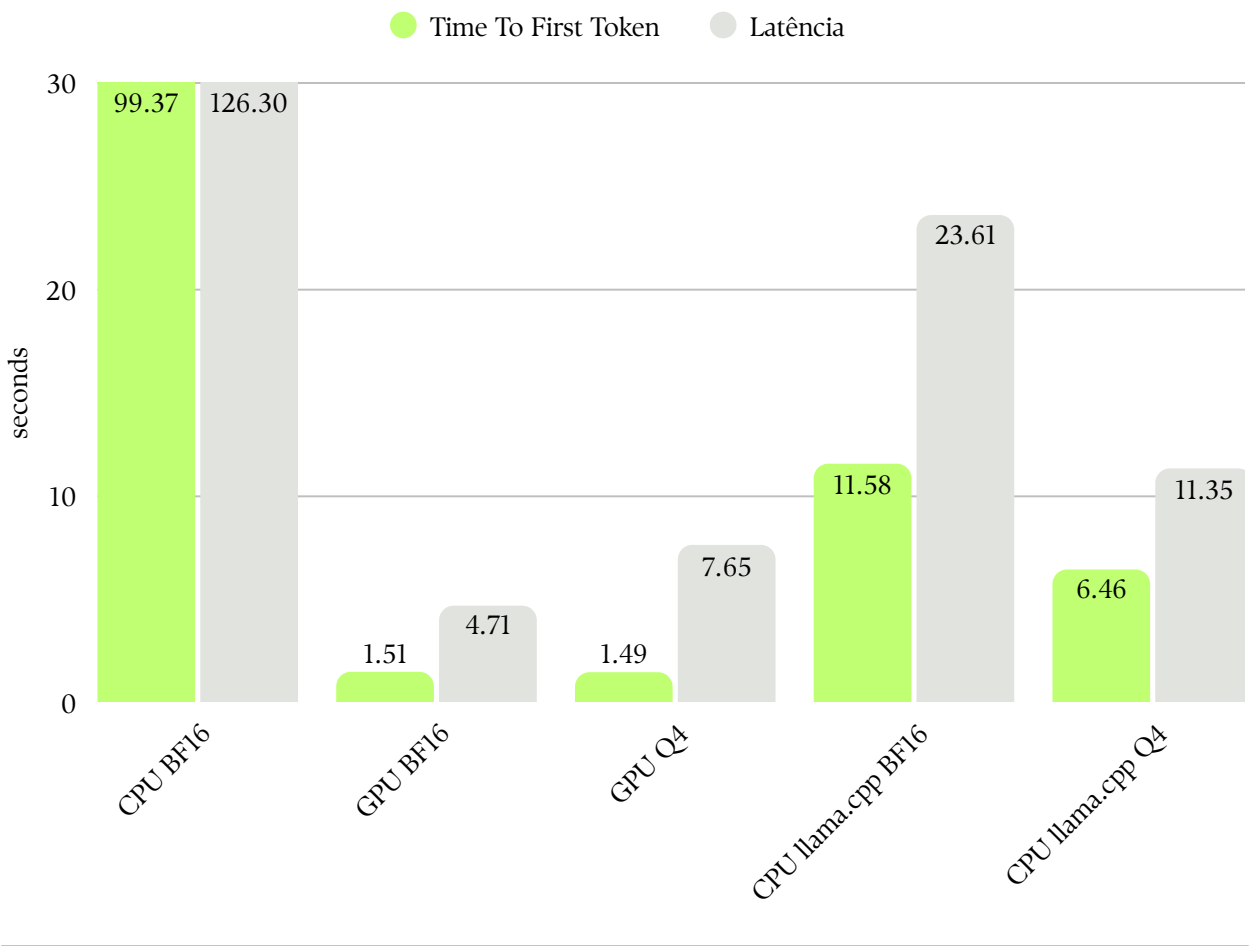
Time Analysis on Qwen3-4B-Base 2k Context
