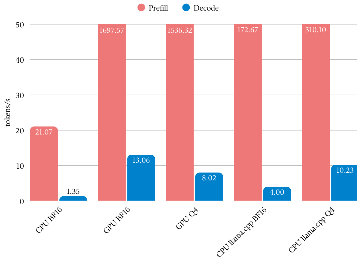
Performance Analysis on Qwen3-4B-Base 4k Context
